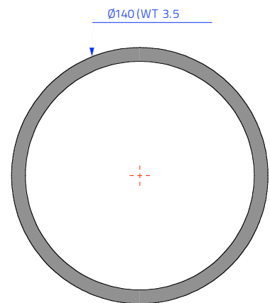
Ø 140 Telescopic Centre Pole Uses: Centre Poles Material: 6261T6 Anodised Aluminium Ultimate Tensile Strength: 295 mpa Yield Strength: 255 mpa
