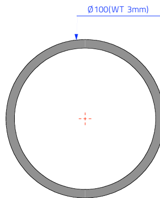
Ø 100 Tube Extrusion Profile Uses: Centre Poles Material: 6261T6 Anodised Aluminium Ultimate Tensile Strength: 295 mpa Yield Strength: 255 mpa
