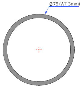
Ø 75 Tube Extrusion Profile Uses: Centre Poles Material: 6261T6 Anodised Aluminium Ultimate Tensile Strength: 295 mpa Yield Strength: 255 mpa
