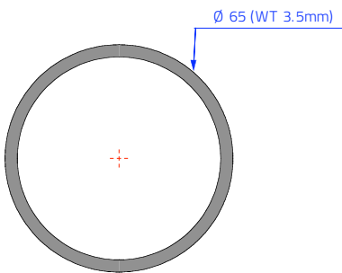
Ø 65 Tube Extrusion Profile Uses: Corner Poles Material: 6261T6 Anodised Aluminium Ultimate Tensile Strength: 295 mpa Yield Strength: 255 mpa
