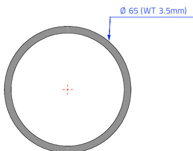
Ø 65 Tube Extrusion Profile Uses: Wall Poles Material: 6261T6 Anodised Aluminium Ultimate Tensile Strength: 295 mpa Yield Strength: 255 mpa
