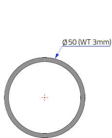
Ø 50 Tube Extrusion Profile Uses: Side & Corner Poles Material: 6261T6 Anodised Aluminium Ultimate Tensile Strength: 295 mpa Yield Strength: 255 mpa
