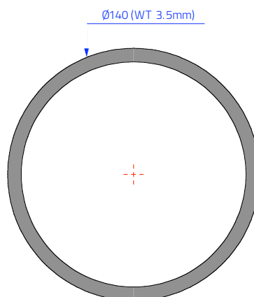
140 Telescopic Centre Pole Uses: Centre Poles Material: 6261T6 Anodised Aluminium Ultimate Tensile Strength: 295 mpa Yield Strength: 255 mpa
