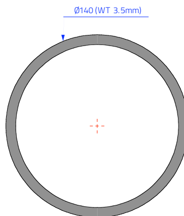
Ø140 Telescopic Centre Pole Uses: Centre Poles Material: 6261T6 Anodised Aluminium Ultimate Tensile Strength: 295 mpa Yield Strength: 255 mpa
