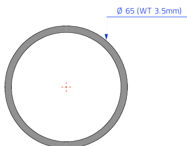
Ø 65 Tube Extrusion Profile Uses: Corner Poles Material: 6261T6 Anodised Aluminium Ultimate Tensile Strength: 295 mpa Yield Strength: 255 mpa
