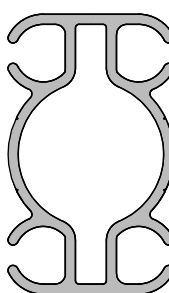
Channel Tube Light 4 Track 83mm x 50mm x 3mm
