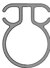
Channel Tube Light 66mm x 49mm x 3mm
