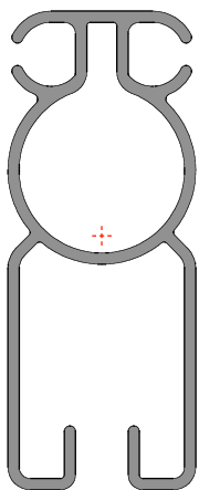
Channel Tube 127mm x 50mm x 3mm
