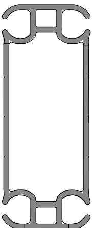
Channel Tube 4 Track 127mm x 50mm x 3mm
