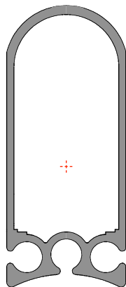
Alirail 112mm x 50mm x 3mm
