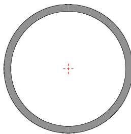
Tube 76.2mmø x 3.25mm
