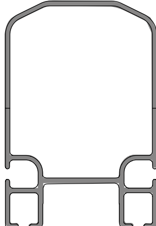
SQ Frame 815mm x 122mm x 2.4mm
