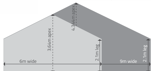
Gable End
